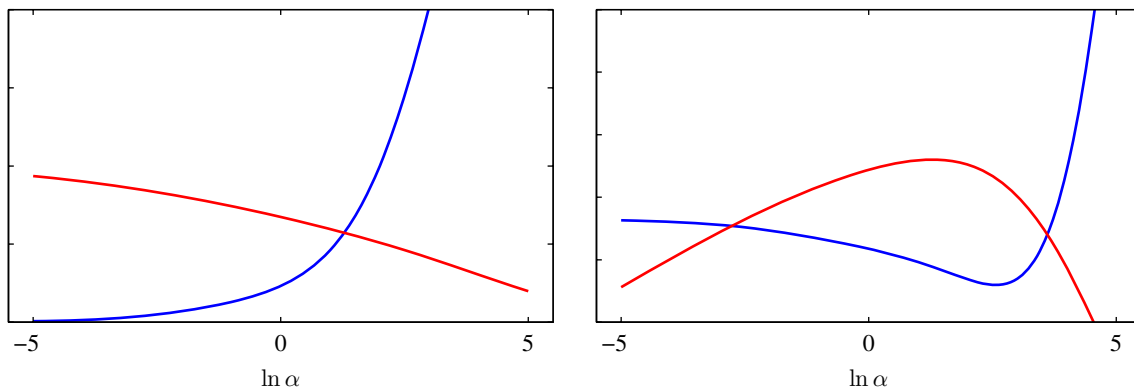
Figure 3.16 The left plot shows \gamma (red curve) and 2\alpha E_W(\mathbf{m}_N) (blue curve) versus \ln \alpha for the sinusoidal synthetic data set. It is the intersection of these two curves that defines the optimum value for \alpha given by the evidence procedure. The right plot shows the corresponding graph of log evidence \ln p(\mathbf{t}|\alpha, \beta) versus \ln \alpha (red curve) showing that the peak coincides with the crossing point of the curves in the left plot. Also shown is the test set error (blue curve) showing that the evidence maximum occurs close to the point of best generalization.
